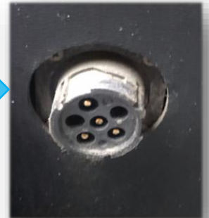
J1708 (6 pin)
